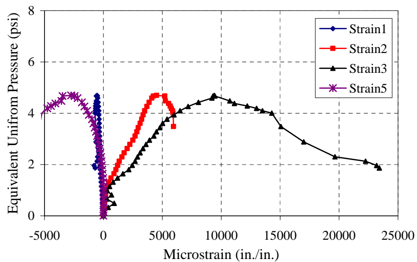
Figure A.1-5. Equivalent Uniform Pressure versus Strain – Wall P1-7
