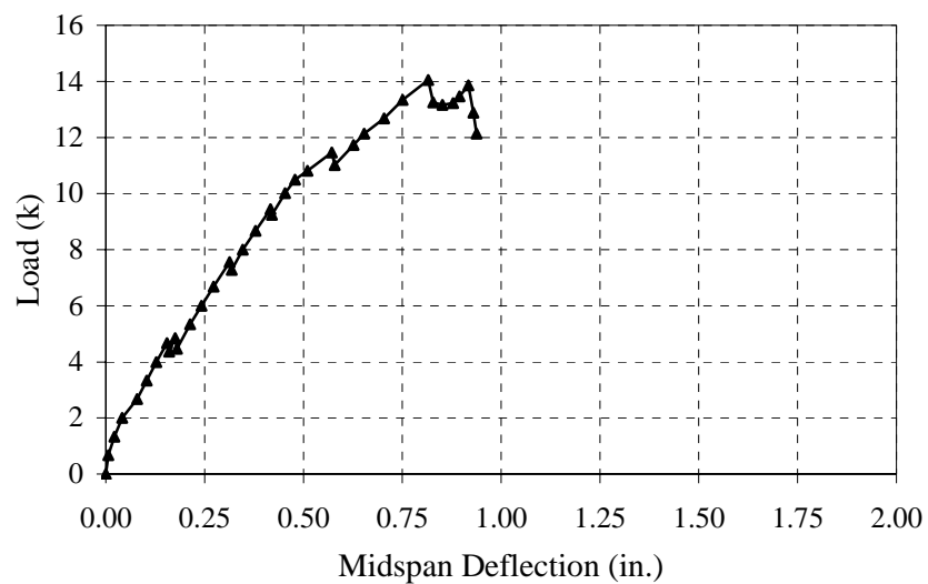
Figure 6.23. Load-Deflection Behavior – Wall P2-7
